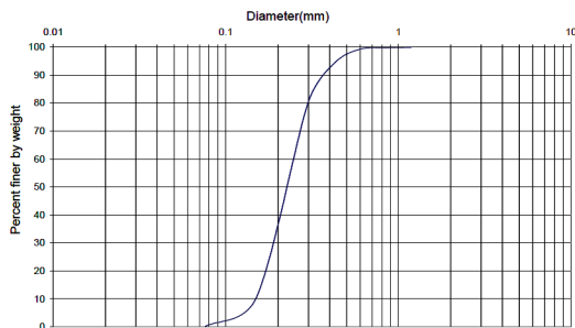
Fig. 6: Diagram of grading sand of study case in Sedghiani & Jiriai's research[7]
