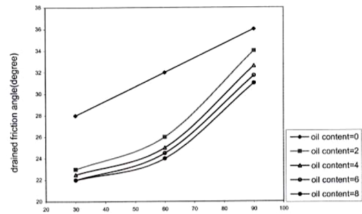
Fig. 8: Diagram of the changes of the angle of internal friction against proportional compression by using CD triaxial test in Sedghiani & Jiriai's study[7]
