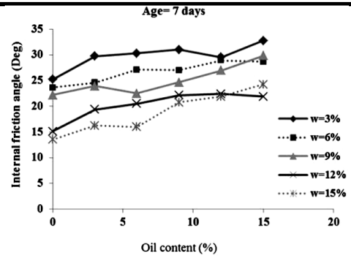
Fig. 2: The effect of the percentage of oil & moisture on the angle of internal friction on 7 days specimens in Kermani & Ebadi's research [5]
