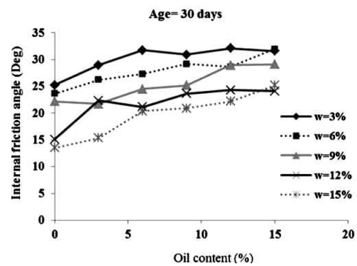
Fig. 3: The effect of the percentage of oil & moisture on the angle of internal friction on 30 days specimens in Kermani & Ebadi's research [5]
