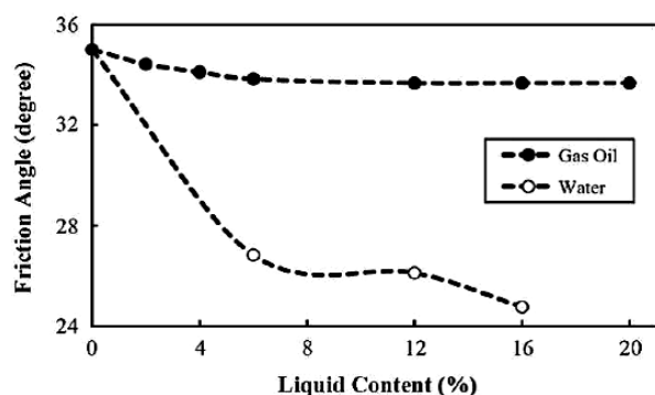
Fig. 9: The effect of the percentage of gas- oil & water on the angle of internal friction of sample of Kaolinite test in Khosravi & co-workers' study[9]
