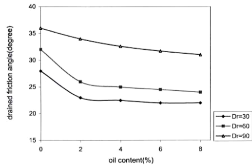
Fig. 7: Diagram of the changes of the angle of internal friction against the percentage of contamination by using CD triaxial test in Sedghiani & Jiriai's study[7]
