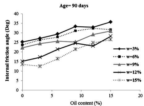
Fig. 4: The effect of the percentage of oil & moisture on the angle of internal friction on 90 days specimens in Kermani & Ebadi's research [5]
