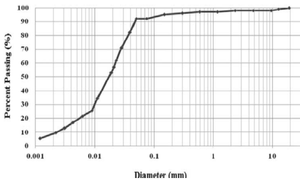
Fig. 1: Diagram of grading soil sample in Kermani & Ebadi's research [5]
