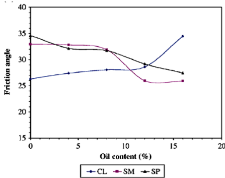
Fig. 5: The percentage Changes of crude oil to the angle of internal friction in Khamehchiyan & colleagues' research[6]
